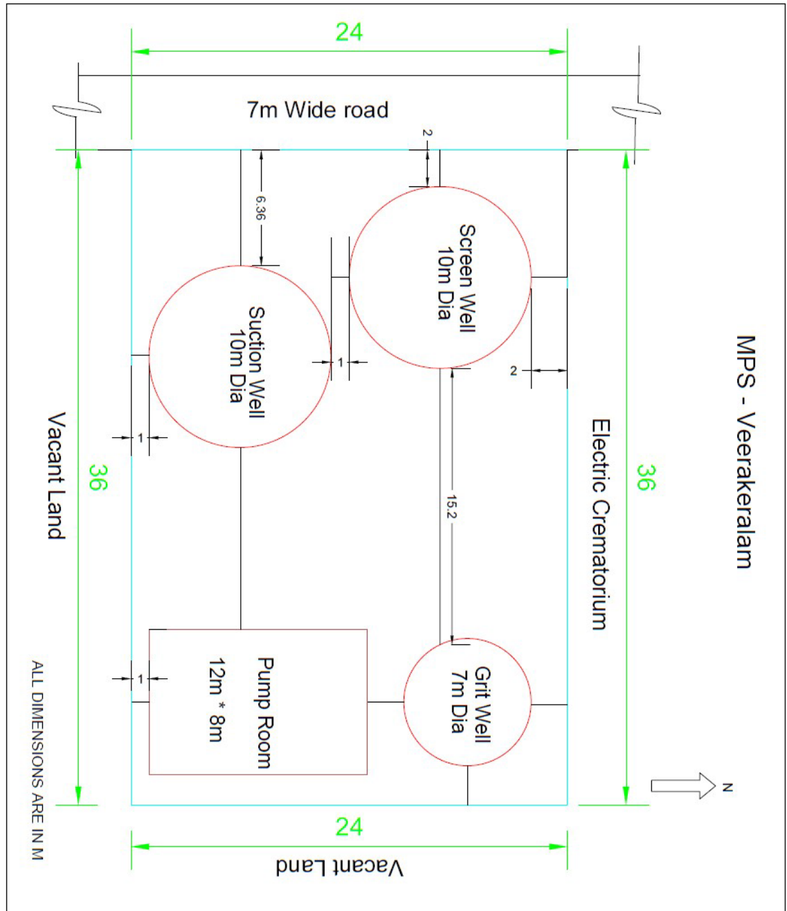
Figure 46: Site Set out Plans-Zone V (MPS - Veerakeralam)
