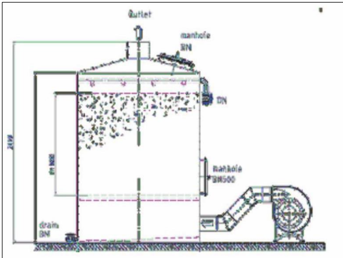
Carbon filter sketch
