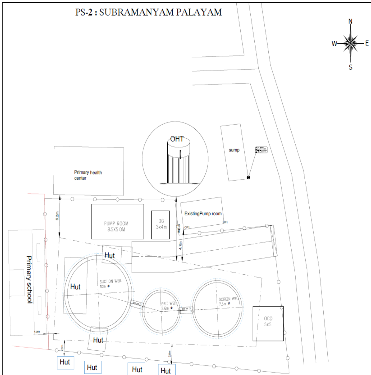
Figure 49: Site Set out Plans – Zone VII (Subramanyam Palayam)
