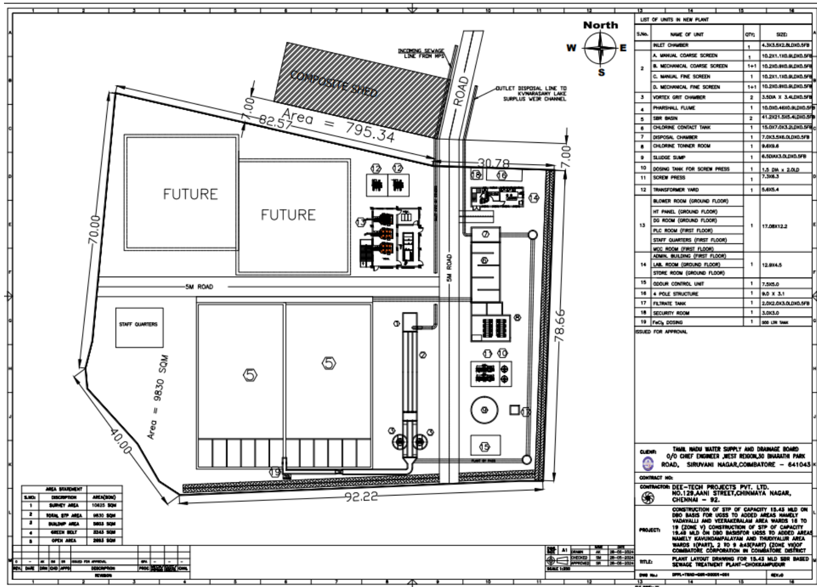
Figure 10 a: Sewage Treatment Plant –Layout
