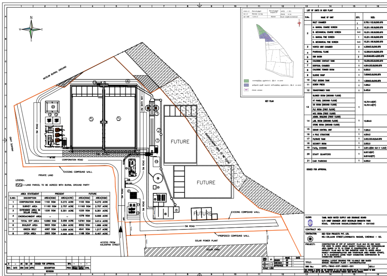
Figure 11 b: Sewage Treatment Plant –Layout
